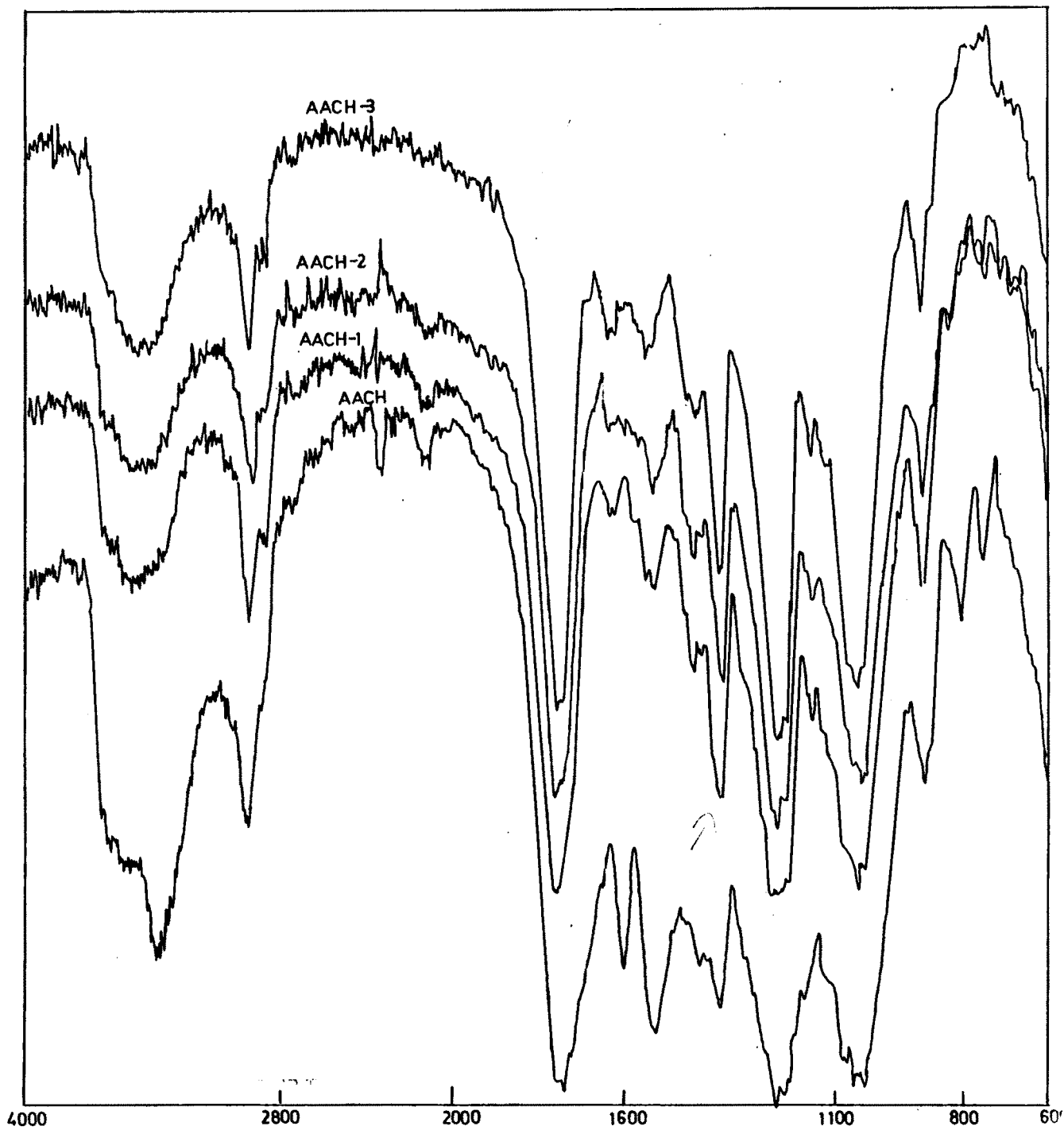
Fig 2 : IR Spectra of AACH Supported Schiff-bases.
