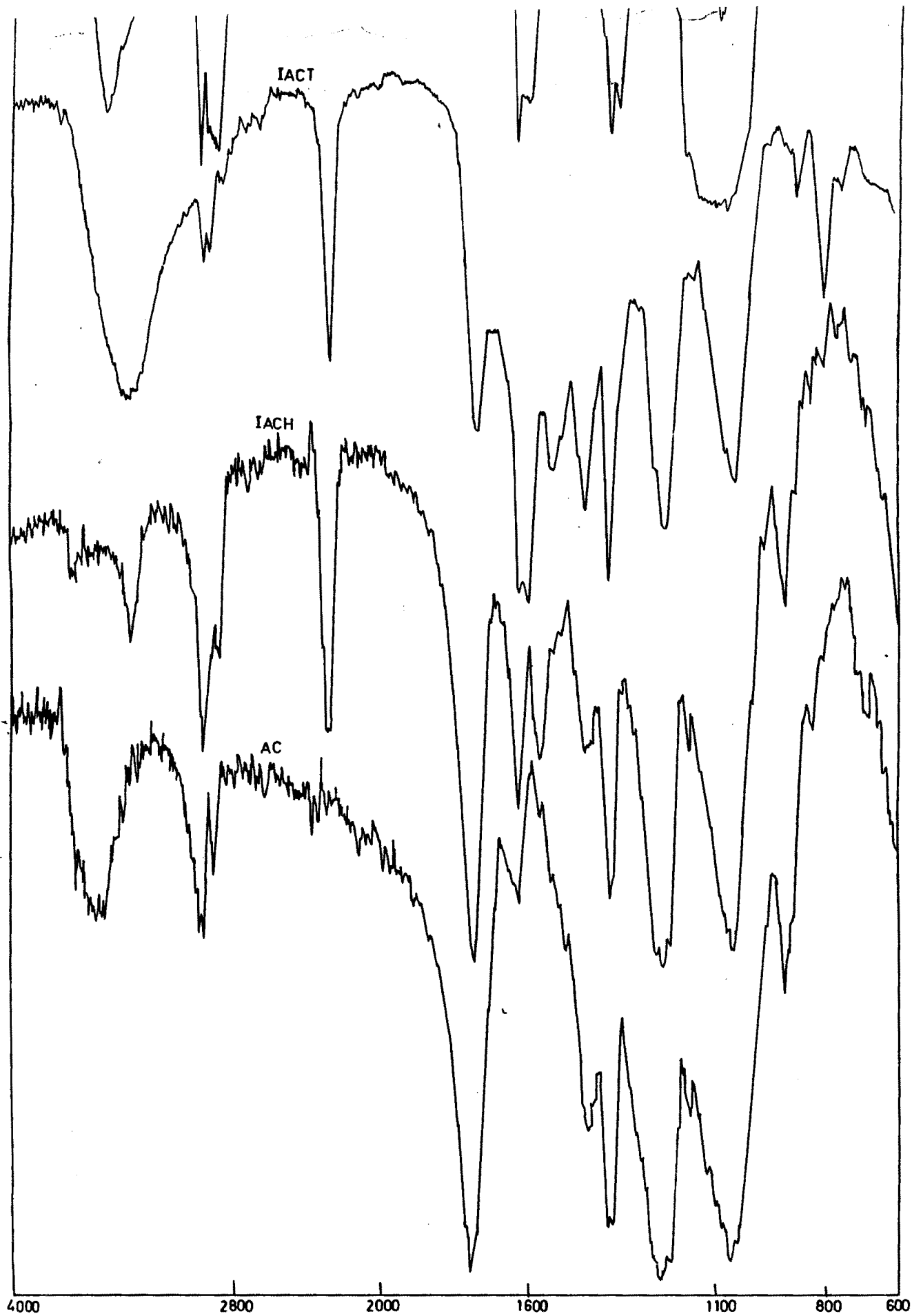
Fig. 1 : IR Spectra of AC, IACH, IACT, EC, IECH, AACH, AACT and AECH compounds.
