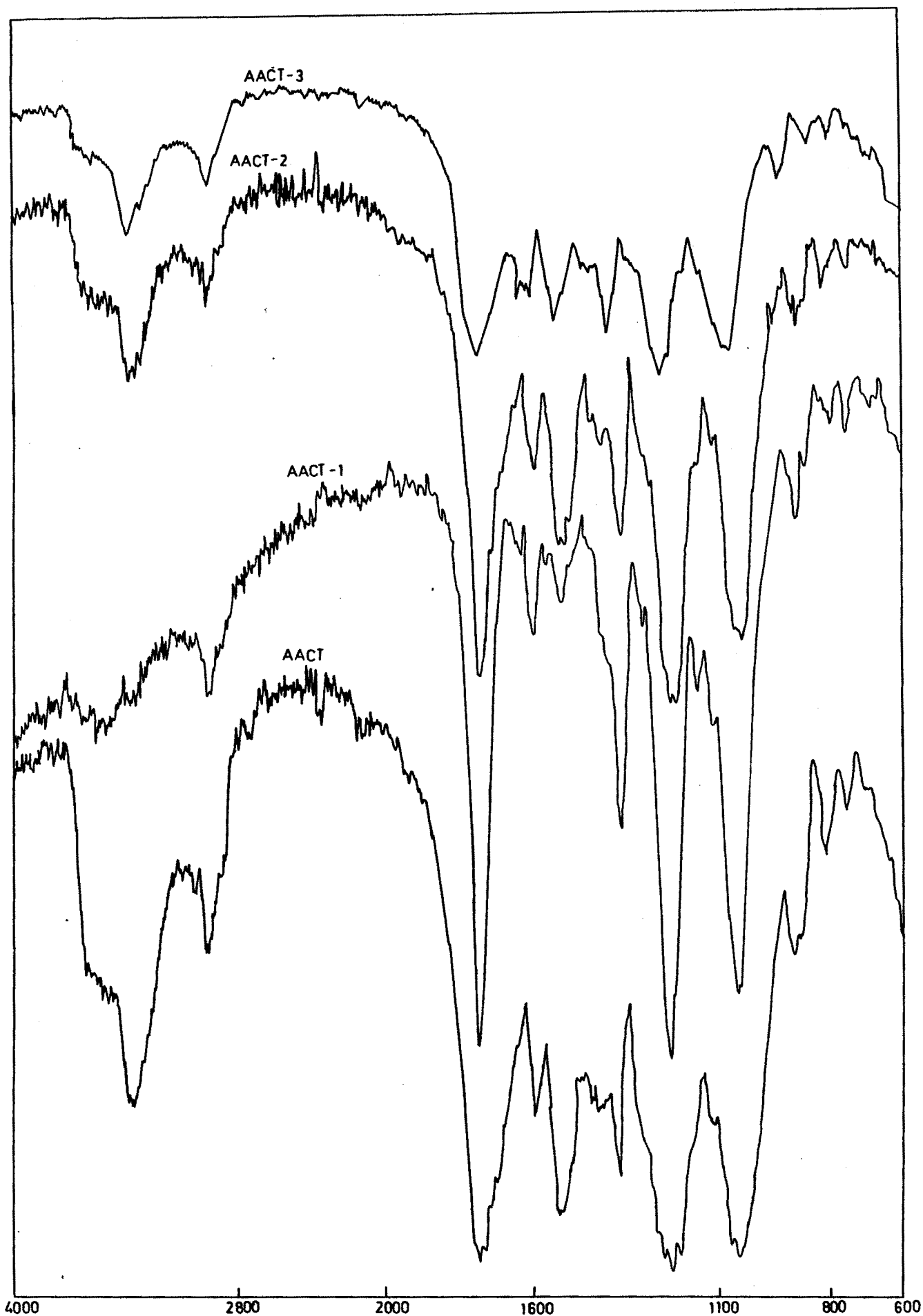
Fig. 3 : IR Spectra of AACT Supported Schiff-bases.
