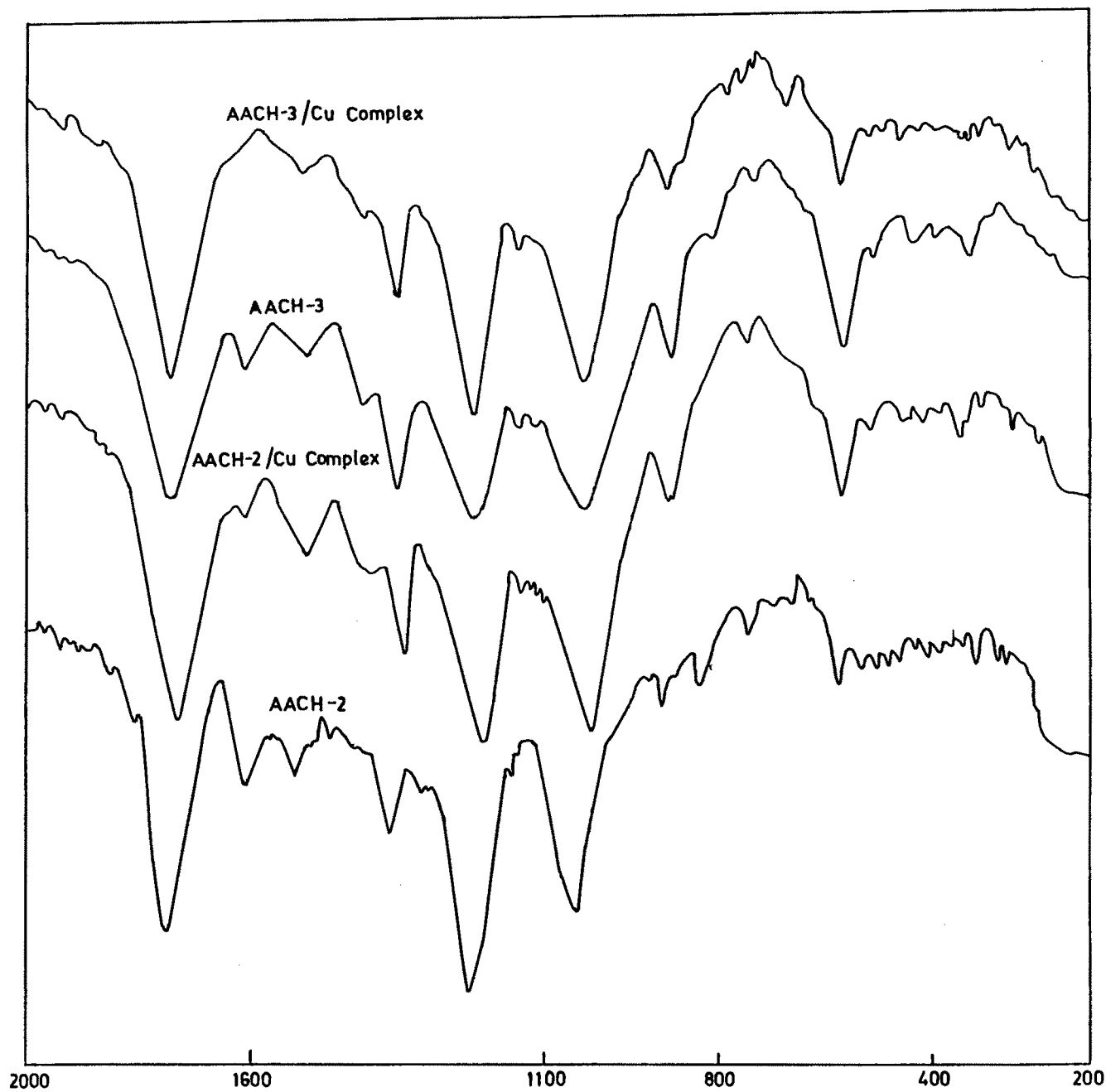
Fig. 7 : IR Spectra of Cu (II) Complex of AACH-2 and AACH-3 Schiff-base.
