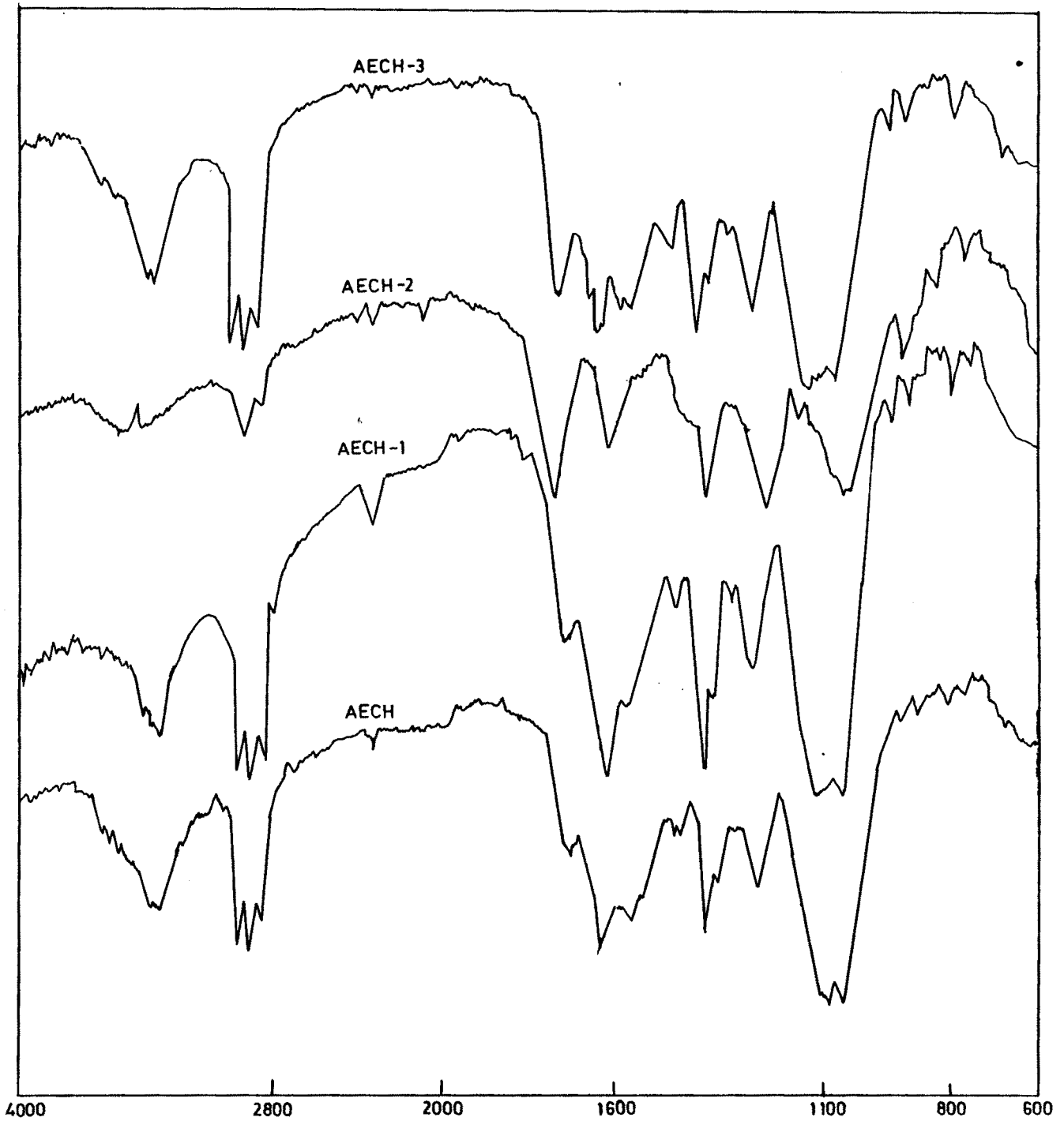
Fig. 4 : IR Spectra of AECH Supported Schiff-bases.
